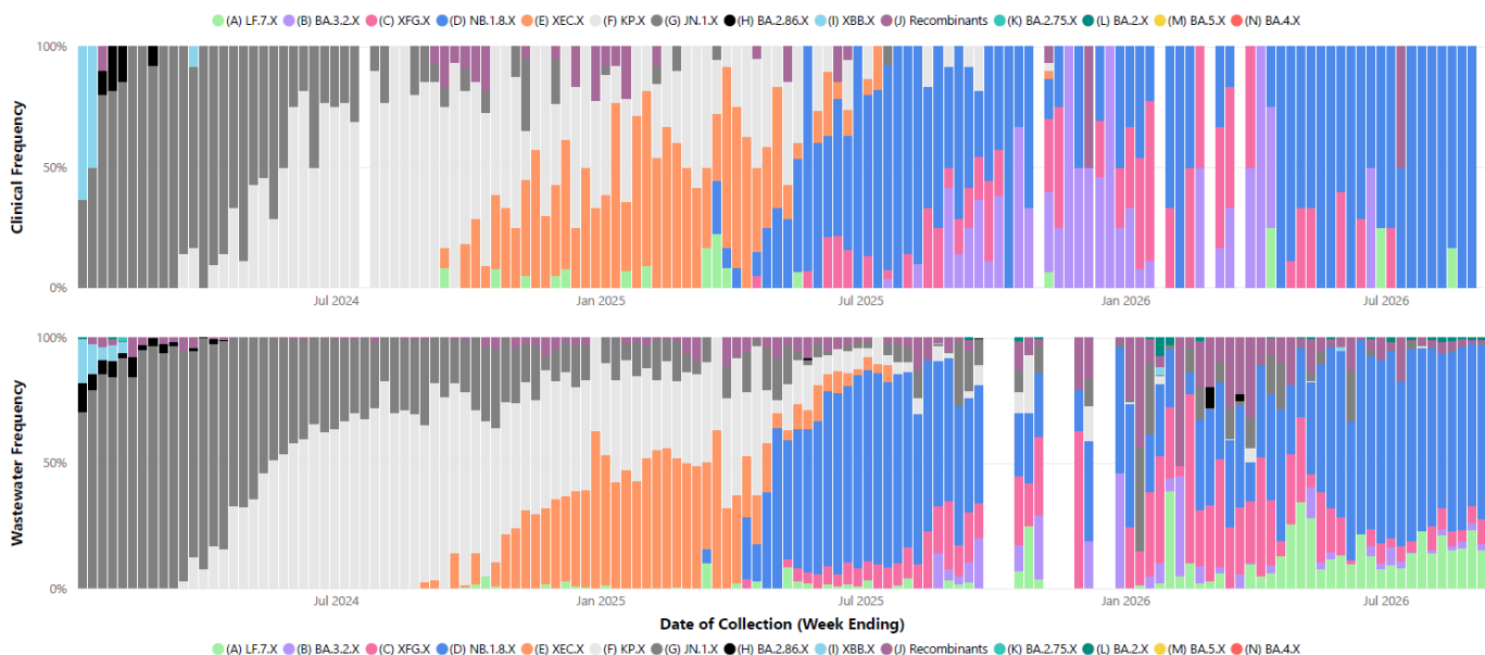
Figure 18. Distribution of SARS-CoV-2 variants in clinical samples (top) and metropolitan wastewater catchments (bottom), 01 Jan 2024 to 6 Sep 2026
