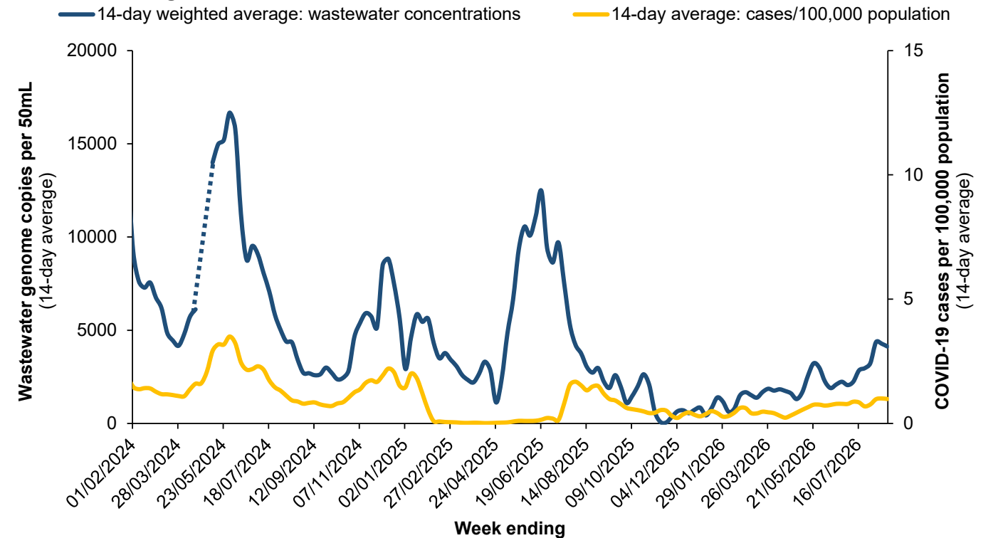
Figure 17. SARS-CoV-2 concentration in wastewater and COVID-19 notification rate, Perth metropolitan area, WA, 2024 to 21 August 2026.
