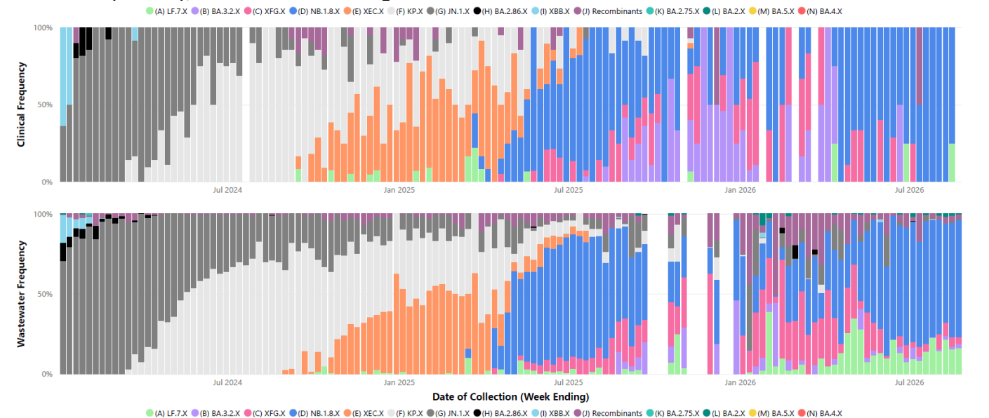
Figure 18. Distribution of SARS-CoV-2 variants in clinical samples (top) and metropolitan wastewater catchments (bottom), 01 Jan 2024 to 23 Aug 2026
